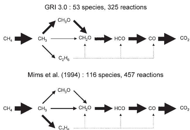
Figure 2. Time-integrated carbon element flux diagrams for mechanism comparison.
